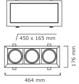
1X3 housing
