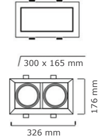
1X2 housing
