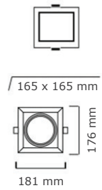
1X1 housing
